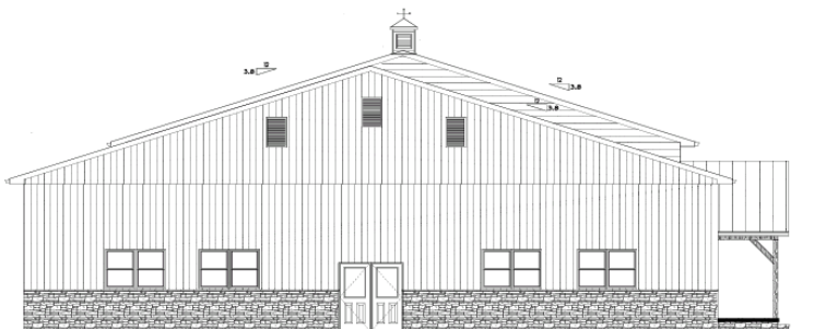
LEFT ELEVATION SCALE: 3/16" = 1'-0"
